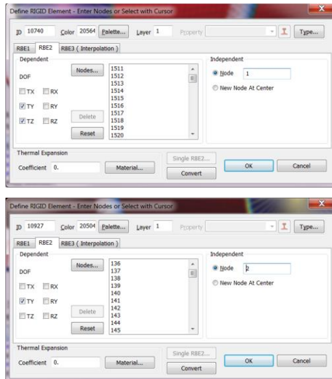
Figure 22: The CBUSH elements with rotational constraints coupled with the RBE2 elements in a cylindrical coordinate system provides a smooth torsion transition along the tube.
