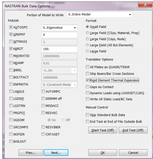
Figure 11: How to setup the RBE2 to handle thermal loading.
