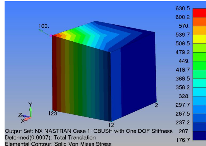
Figure 18: The CBUSH nodes are coincident and the load case is a 100 lbf vector load in 1,1,1 direction. The CBUSH element is stable.
