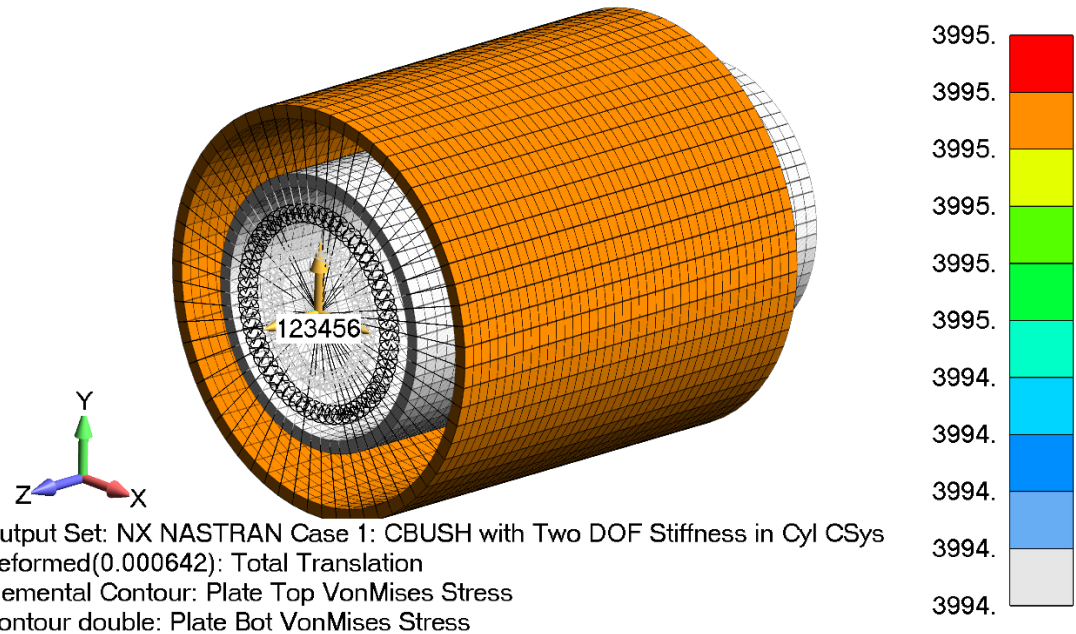
Figure 26: Using the CBUSH Element to obtain the same result as shown for the RBE3 and RBE2 connections.
