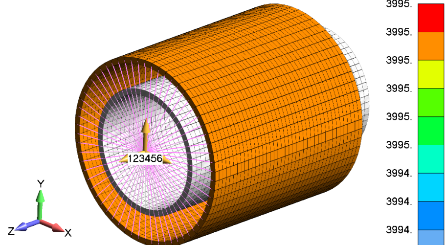
Output Set: NX NASTRAN Case 1: RBE2 in Cyl CSys Deformed(0.000642): Total Translation Elemental Contour: Plate Top VonMises Stress Contour double: Plate Bot VonMises Stress
