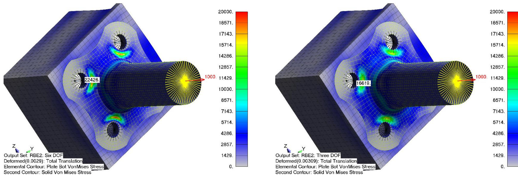
Figure 5: A column is pulled with a force of 1,000 lbf. A RBE3 is used to uniformly distribute the load. RBE2's are used to simulate a bolted connection to the base structure.
