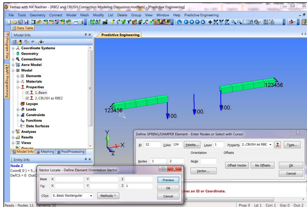
Figure 14: Femap setup for the CBUSH element. Even though the CBUSH property card was set to use Cartesian CSys, the element definition still requires an Element Orientation Vector (viz., just like a beam element).
