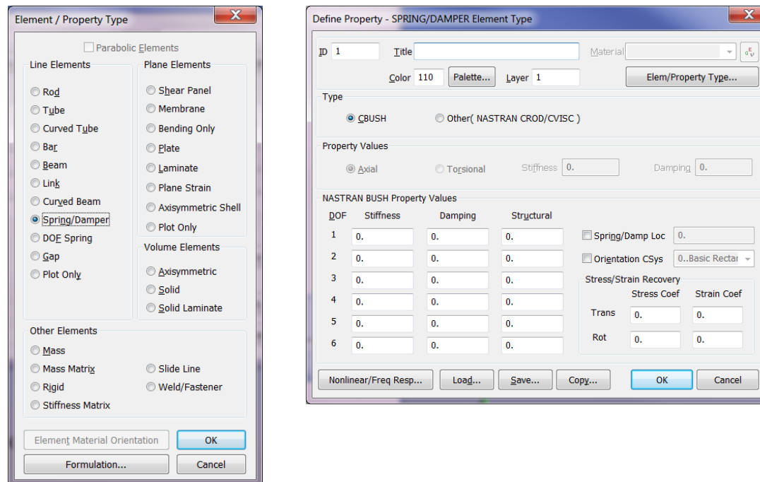
Figure 12: The CBUSH element setup within Femap v11. The column labeled Structural refers to Structural Damping.
