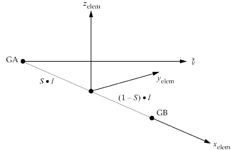
Figure 12-16. CBUSH Element
