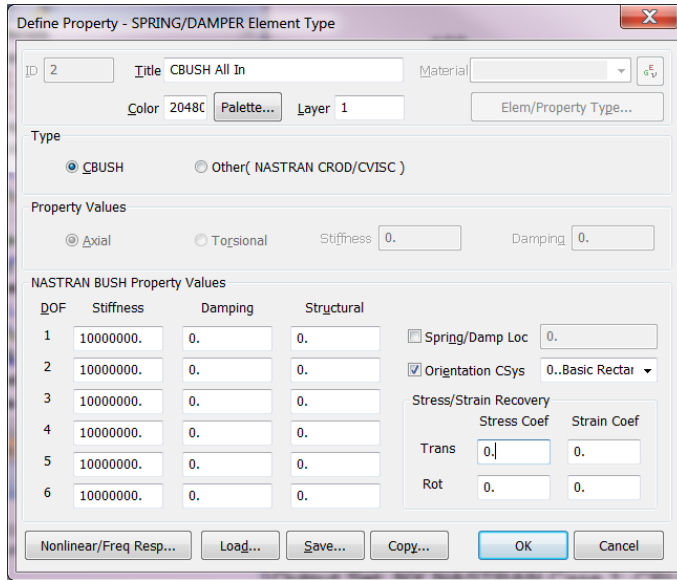
Figure 20: With the end node of the CBUSH constrained in RX, RY and RZ, the element is stable.
