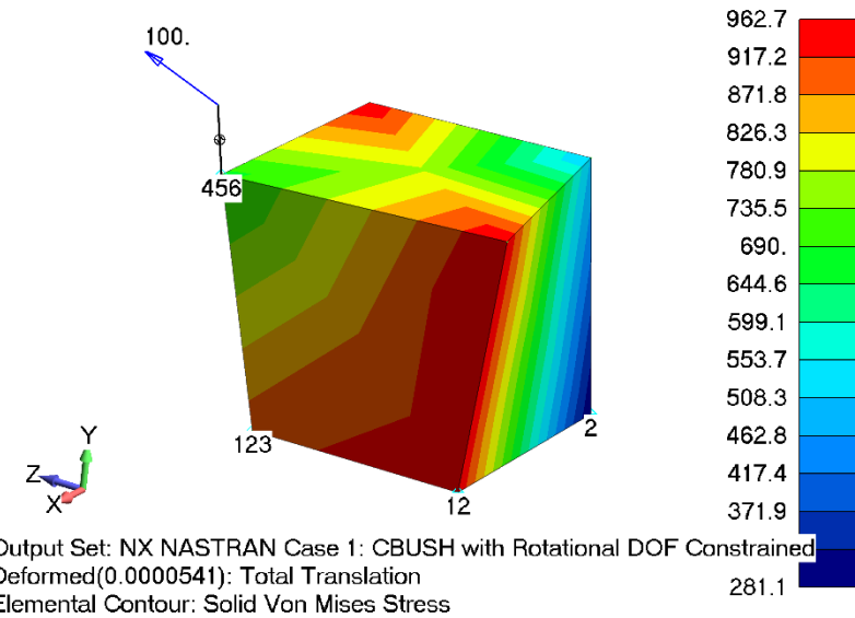
Figure 20: With the end node of the CBUSH constrained in RX, RY and RZ, the element is stable.
