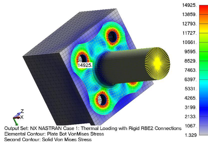
Figure 10: Result of using a rigid RBE2 for thermal analysis. Note: The only applied load is that of a uniform temperature.
