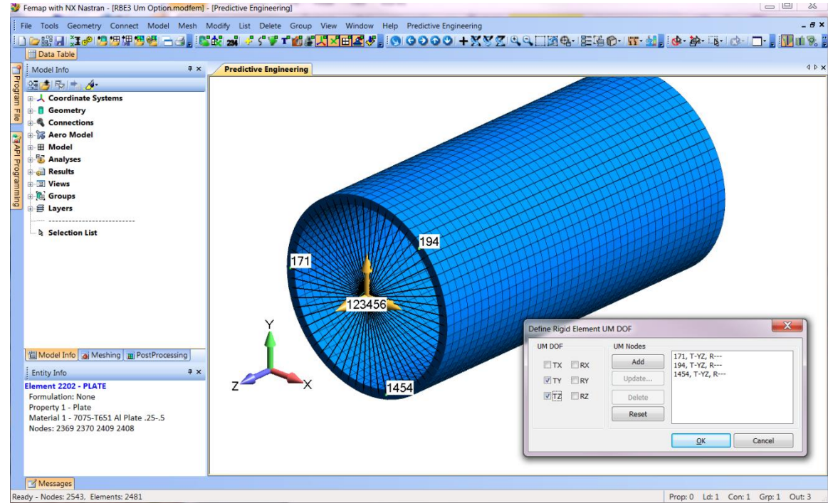
Figure 24: Setting up the RBE3 with the Um option to provide restraint to the internally pressurized cylinder.
