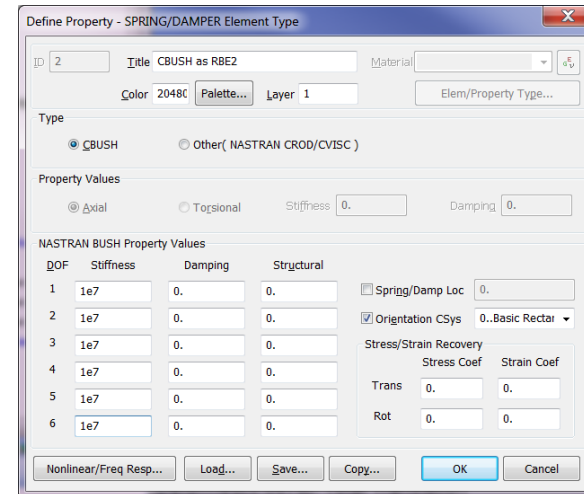
Figure 15: Comparison between RBE2 and CBUSH connection modeling. It is best said that there is no free lunch since the CBUSH element does not quite provide “rigid” type results, unless one uses high stiffness values, which could then lead to numerical problems.
