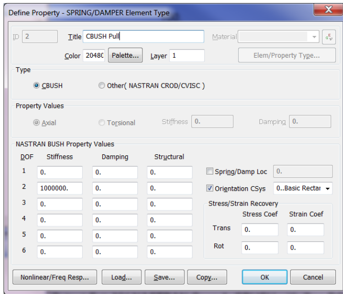
Figure 17: The obvious setup for a CBUSH element attached to a solid element where the load is vertical (Y-direction).
