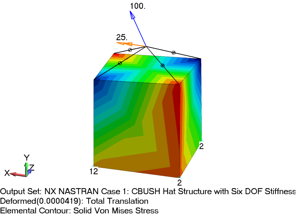
Figure 21: With a stable arrangement, the CBUSH can transfer moment loads onto solid elements; however, the stiffness of the CBUSH element is likewise transferred unlike the RBE3.
