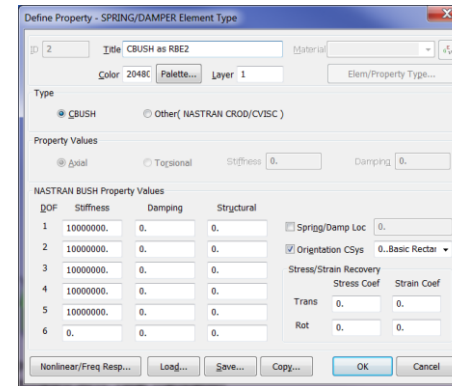
Figure 16: Another comparison between a RBE2 and CBUSH connection element. The CBUSH element does not create a rigid mechanism.
