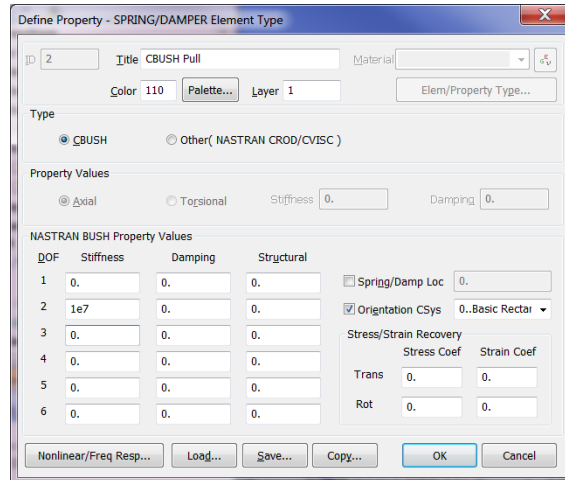
Figure 18: The CBUSH nodes are coincident and the load case is a 100 lbf vector load in 1,1,1 direction. The CBUSH element is stable.
