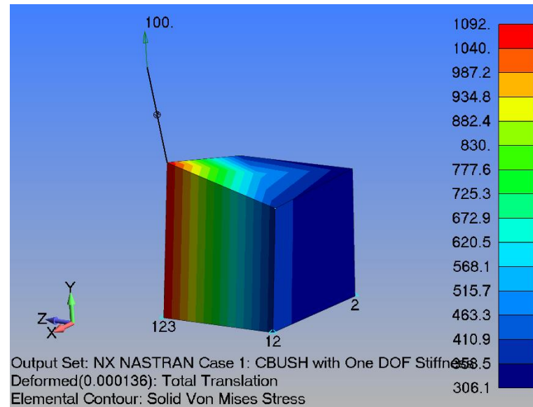
Figure 17: The obvious setup for a CBUSH element attached to a solid element where the load is vertical (Y-direction).
