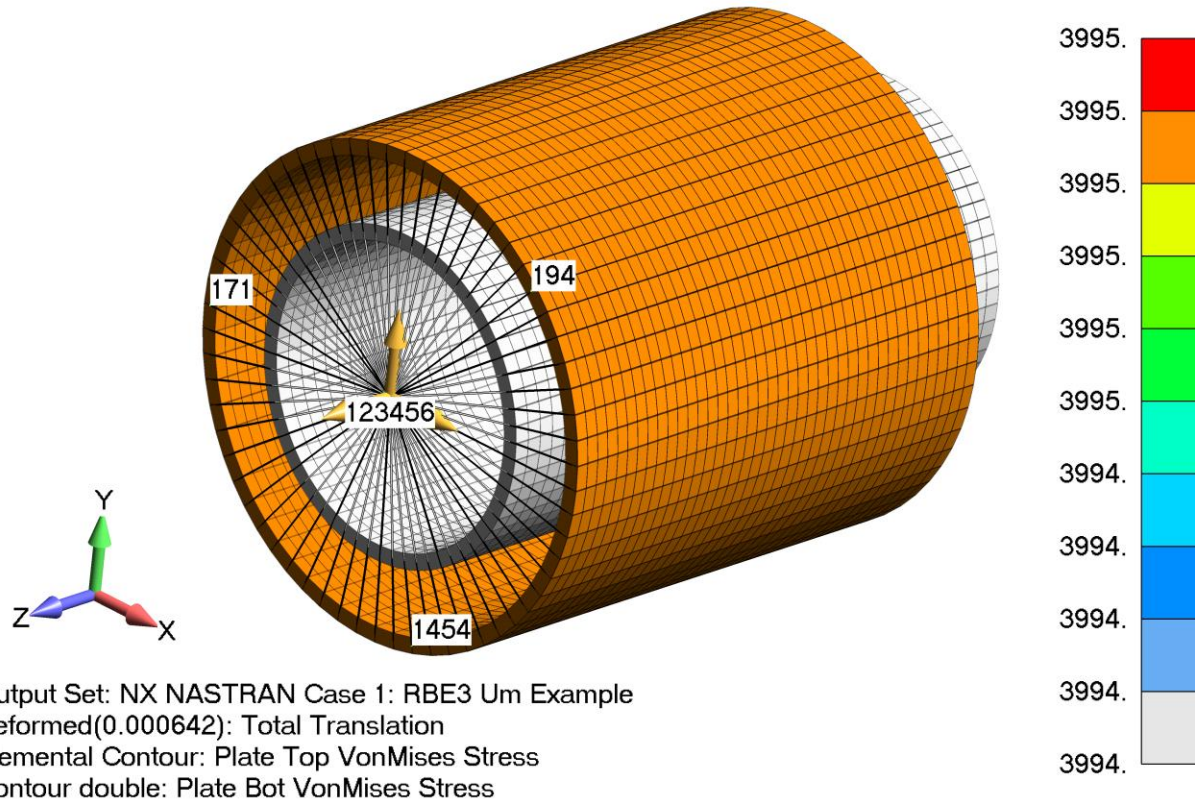
Figure 23: An internal pressure is applied to the cylinder. The RBE3 provides constraint without rigidity. The dependent node is SPC'ed in all six DOF at the center. This is impossible without transferring these SPC's to the U_m DOF.
