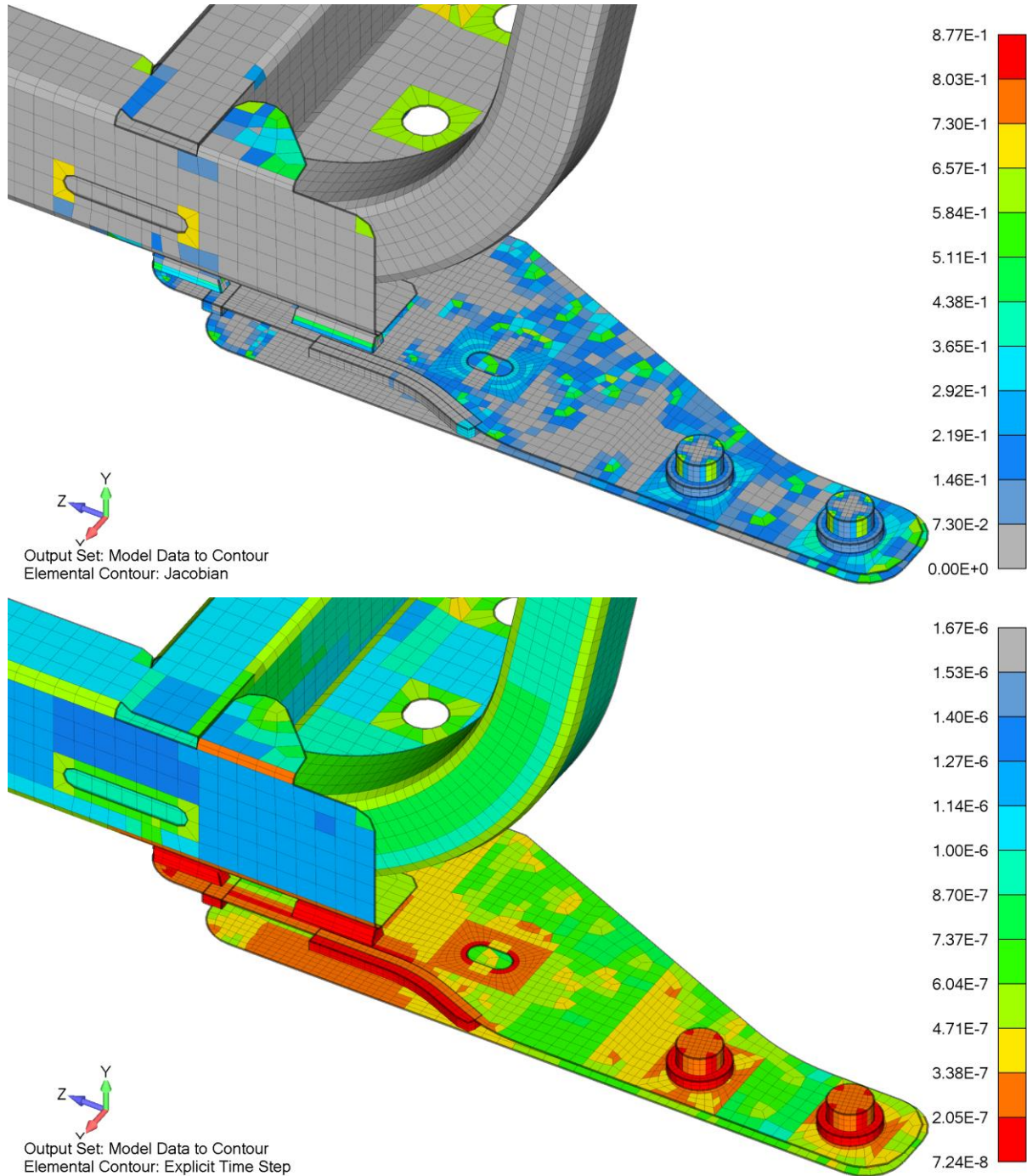
Fig.2: Finite element mesh quality (Jacobian) and explicit time step
