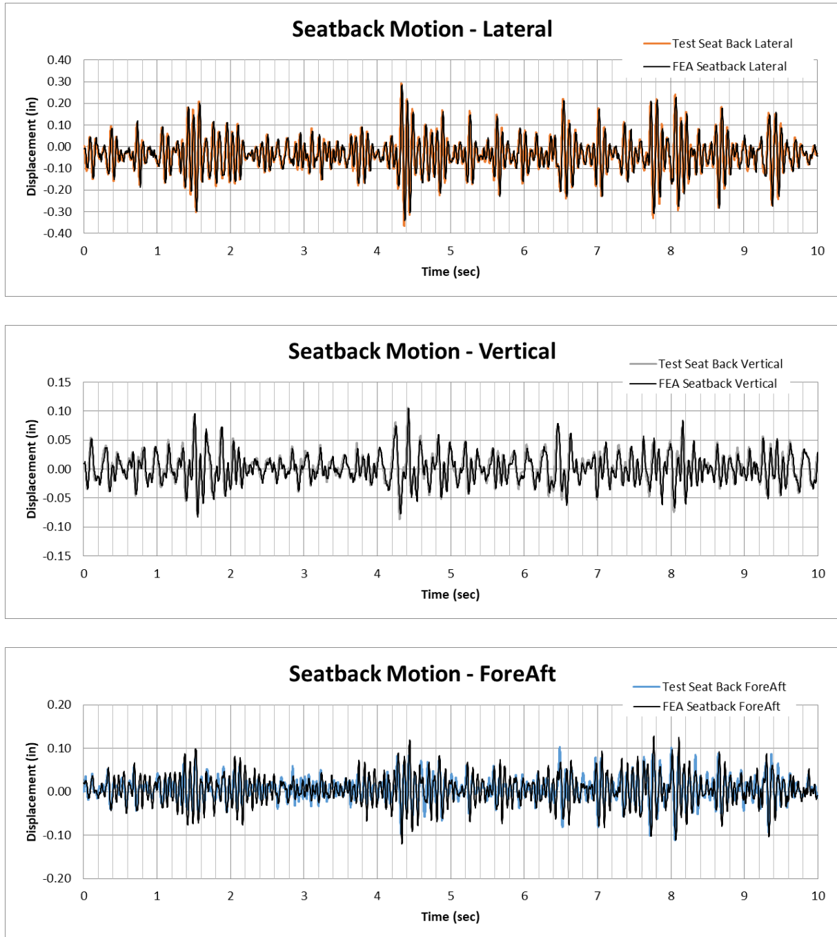
Fig.10: Seatback motion – physical test data vs. FEA results.
