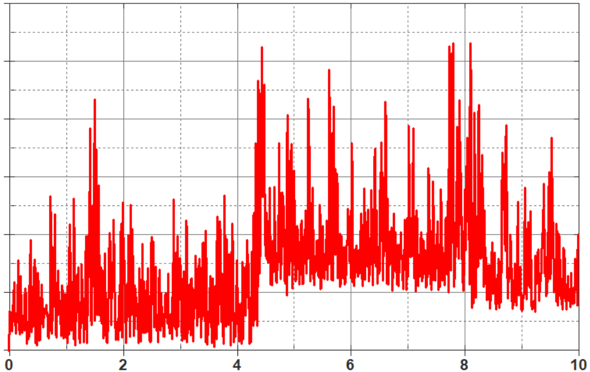
Fig.8: Nonlinear transient stress development during 10 analysis second run
