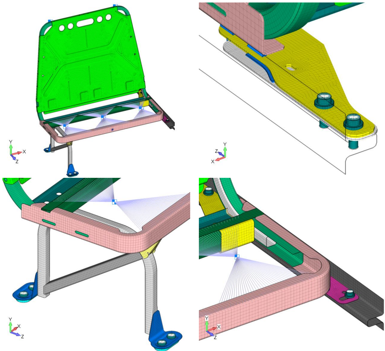
Fig.1: Typical finite element mesh for a bus seat model
