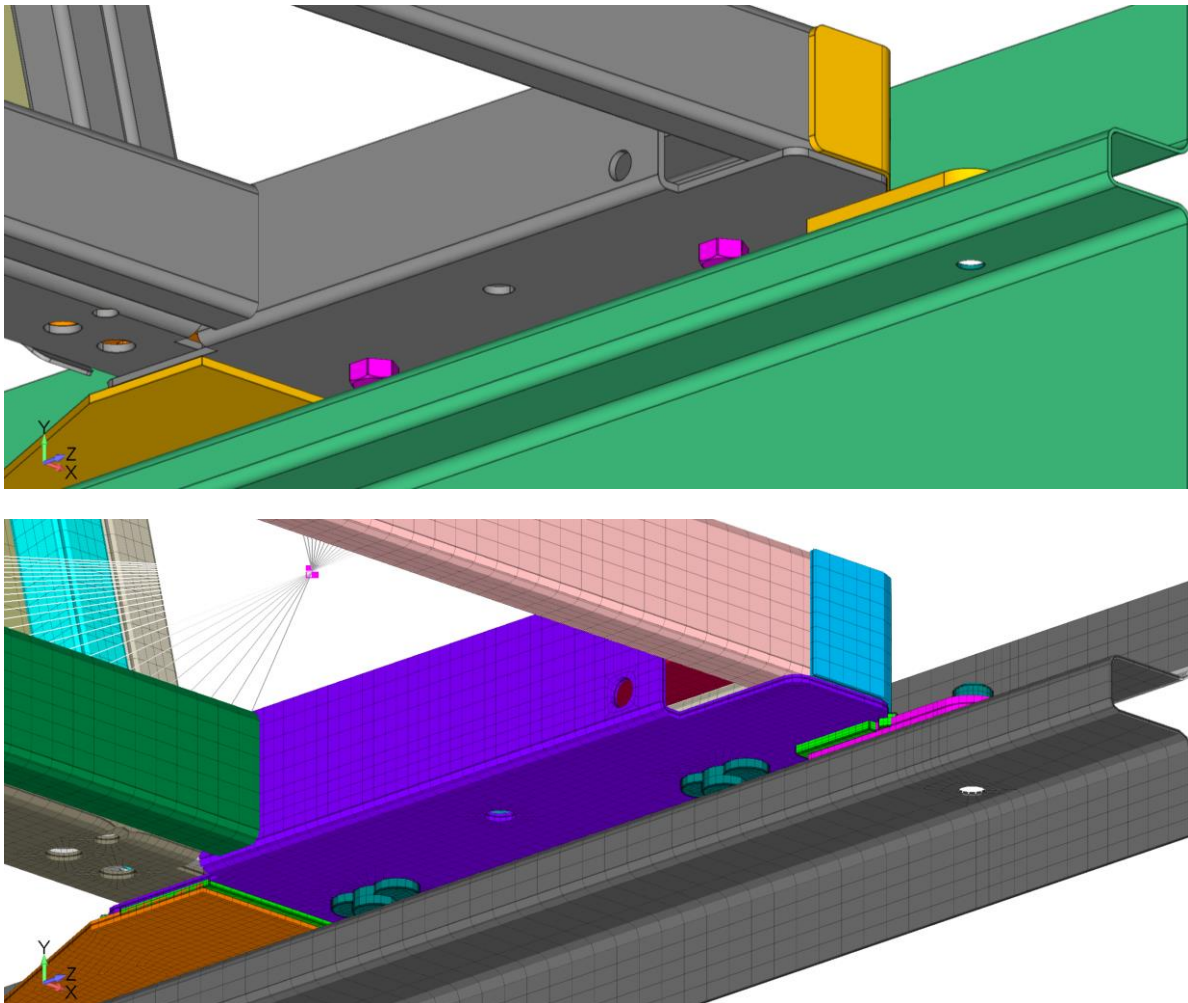
Fig.6: Separating contact interface
