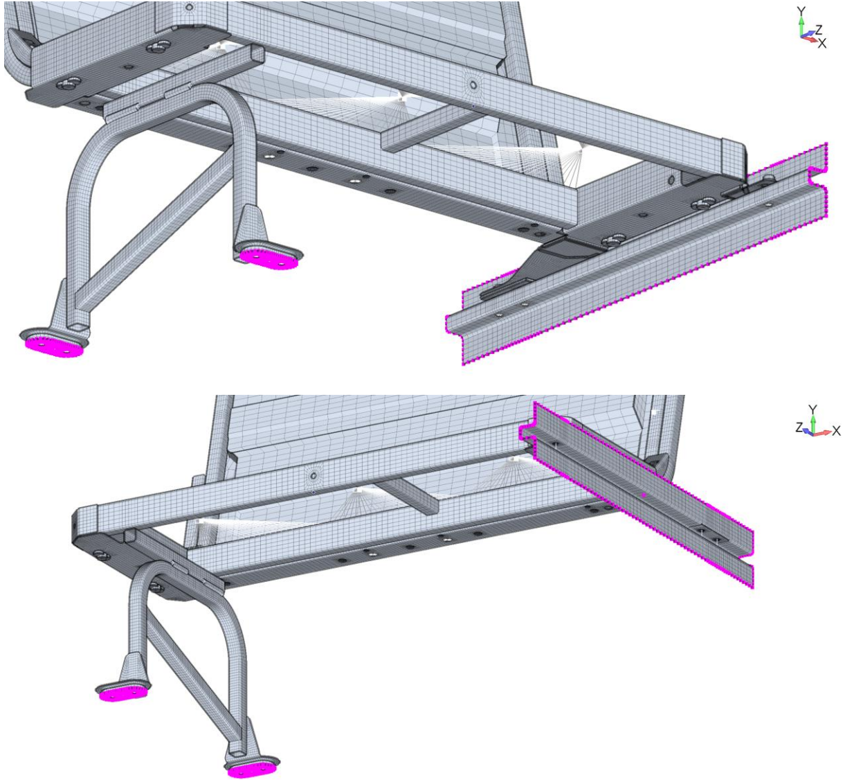
Fig.3: Longitudinal, lateral and vertical displacement inputs for the feet and wall
