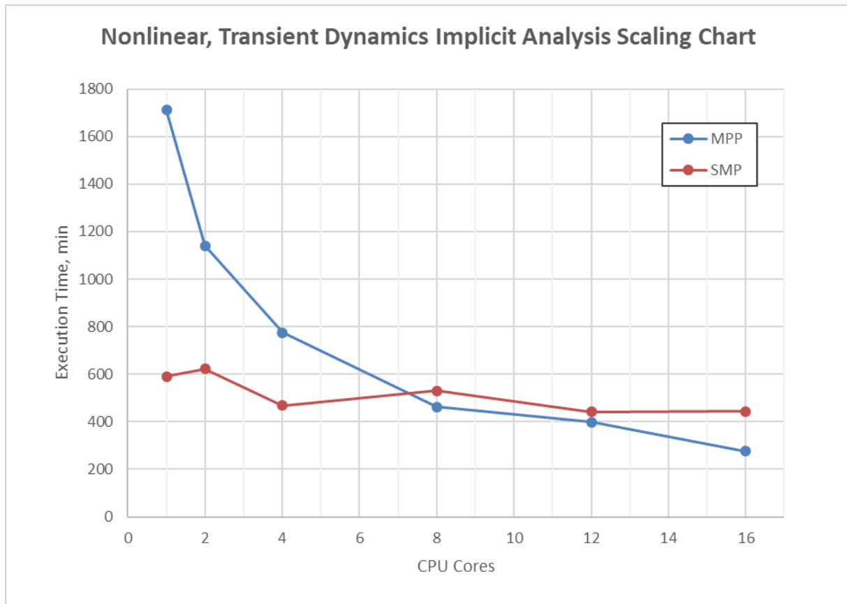
Fig.9: Nonlinear transient dynamics – implicit analysis scaling
